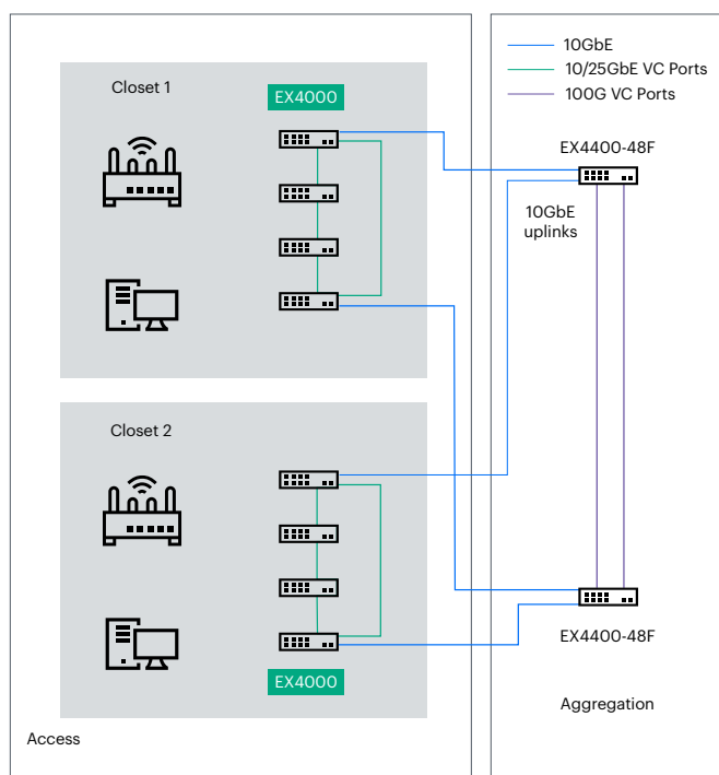
Figure 3: EX4000 Virtual Chassis config interconnected via dedicated front-panel 10GbE ports
